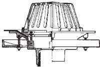
Deck Clamp
